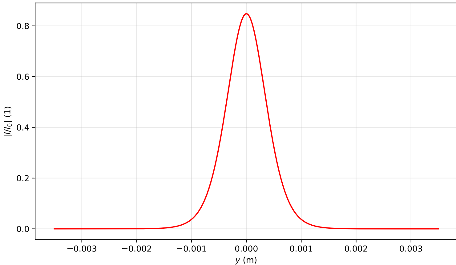
Intensity profile I(x = 0, y, z = 1.911)/I_0 , P_{in}=0.5P_{cr} , artificial time
